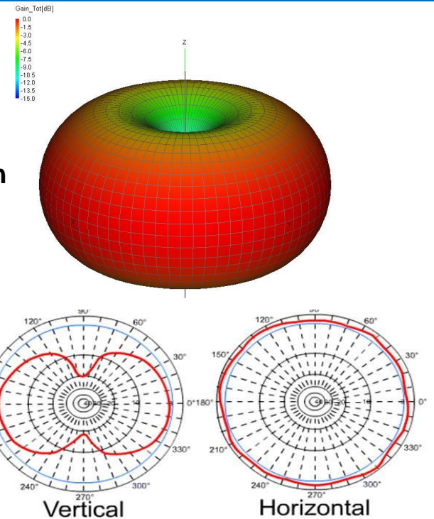
Typical Radiation Pattern Polar Plot
